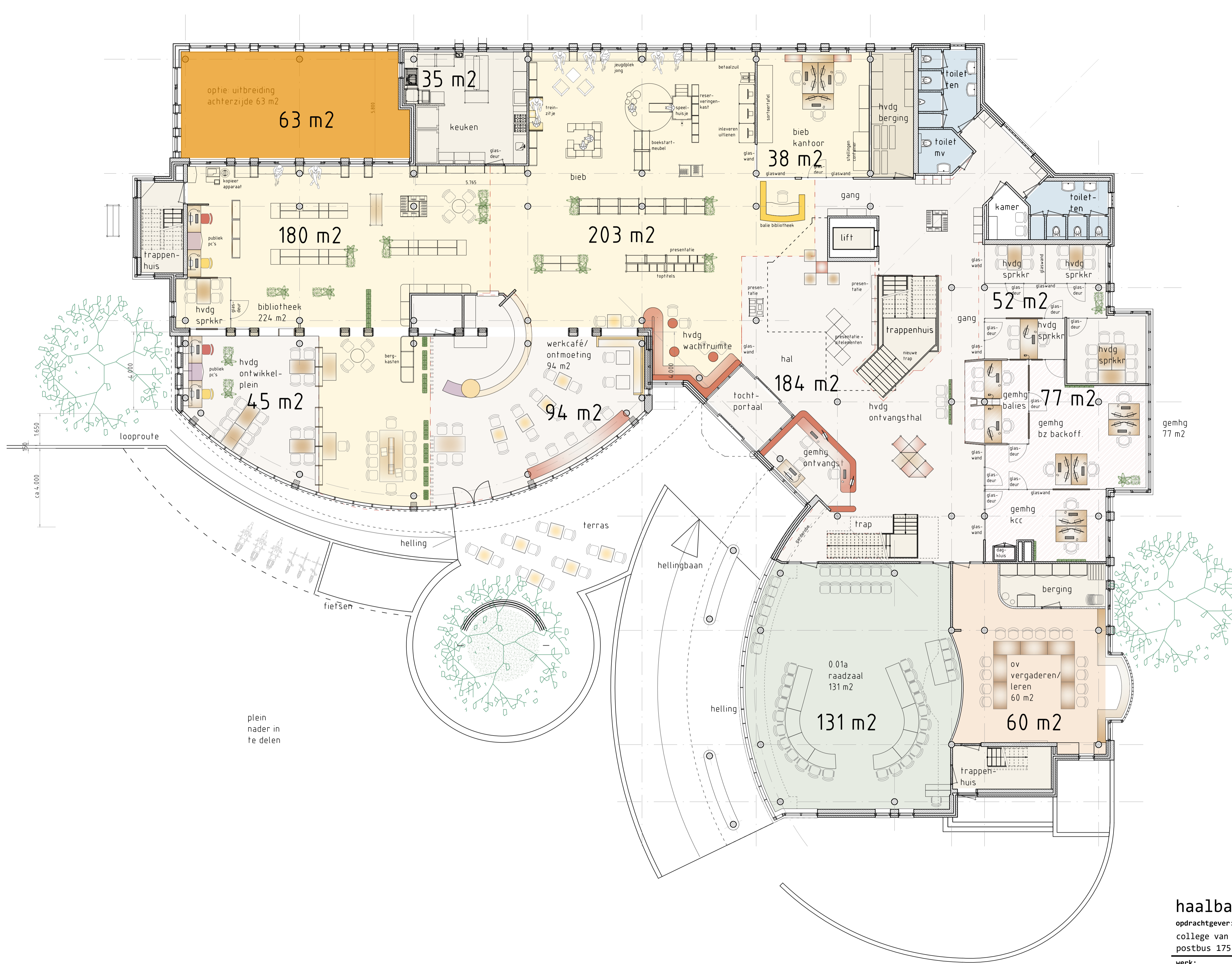
begane grond variant 3a
