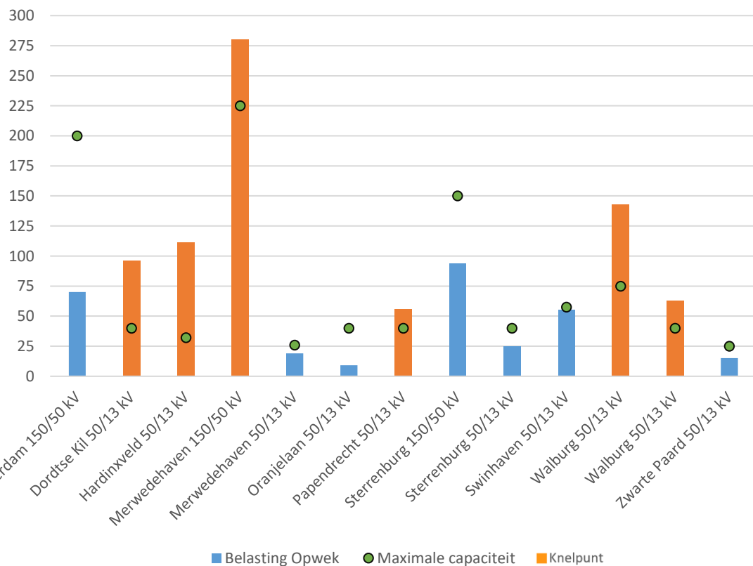
Belasting door opwek per station - Hoog
