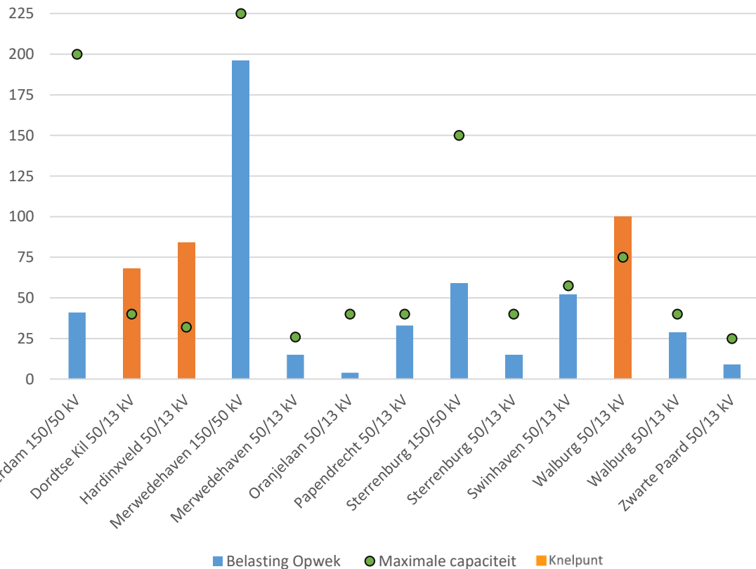
Belasting door opwek per station - Midden
