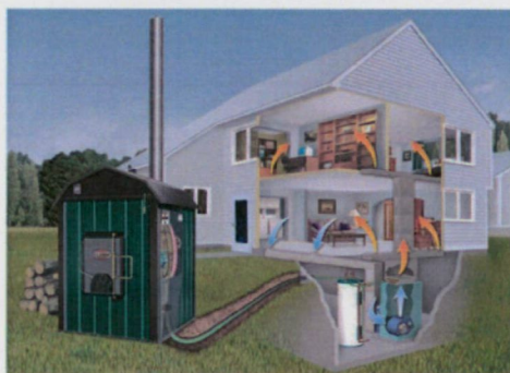
Fig. 2. Hydronic heater integrated with heating system. Shown here is the unit integrated with a forced hot air furnace, but other integrations may include radiant floors, radiators, or baseboards [30].
